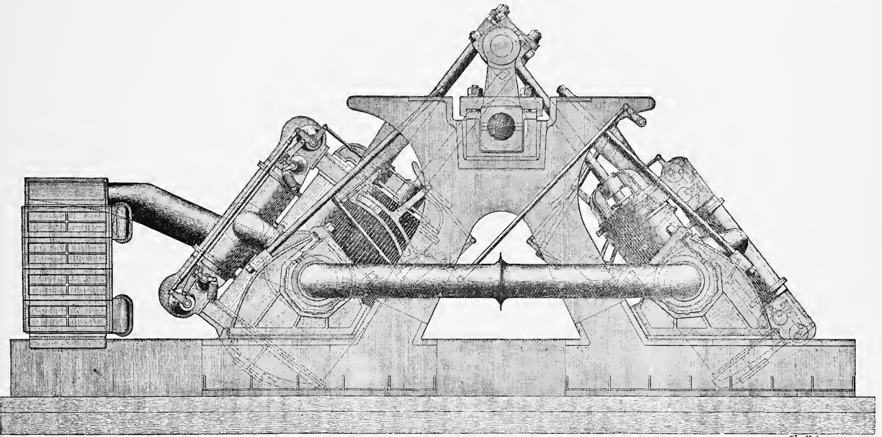
COMPOUND OSCILLATING ENGINE OF THE PROVIDENCE AND STONINGTON LINE STEAMER CONNECTICUT. —Built by Wm. Cramp & Sons, Philadelphia, Pa.
